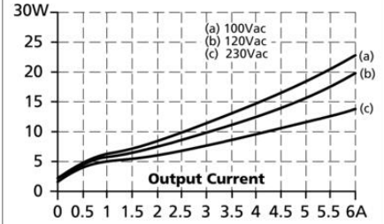
Power Losses
