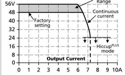
Output Voltage
