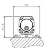
Bottom fixing bracket mounting
