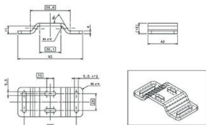
Bottom fixing bracket mounting
