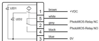
Connection diagram and connector M8, 5-pole
