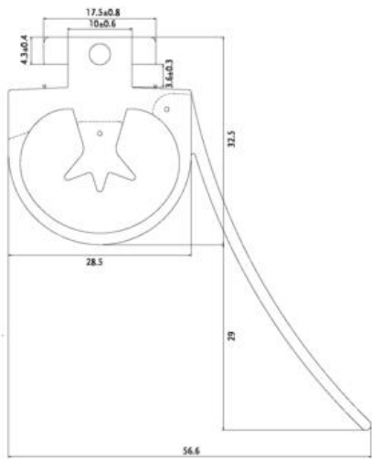
Profile cross-section Contact-Duo 3100.0510B
