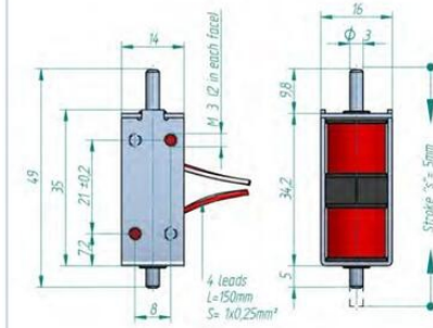
Dimensional drawing:
