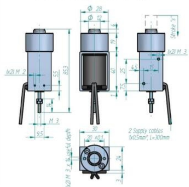
Solenoid shown under voltage
