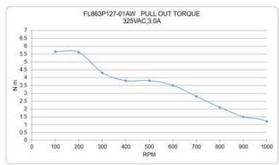
Torque Curve
