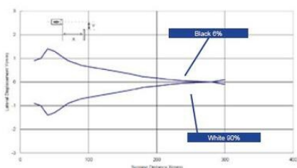
DETECTION AREA - BACKGROUND SUPPRESSION
