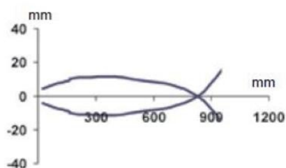
DETECTION AREA - DIFFUSE PROXIMITY
