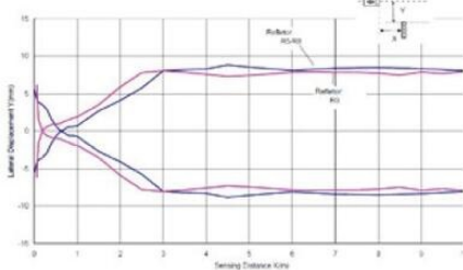
DETECTION AREA - POLARISED RETROREFLEX
