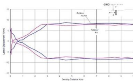
DETECTION AREA - POLARISED RETROREFLEX
