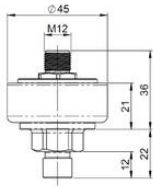
981 with threaded connection
