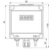
Duct connection for Climaset® 6550/6556
