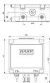
Duct connection for Climaset® 6556/6556
