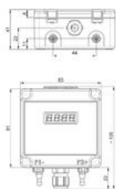
Duct connection for Climaset® 6556/6556
