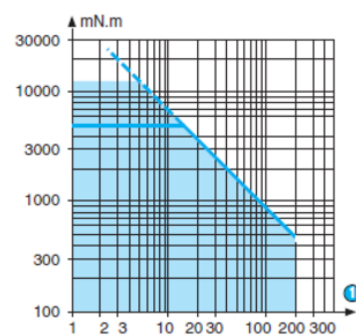
Curve: torque/nominal speed 808070
