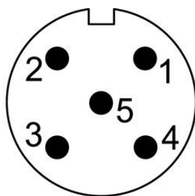
M12 5-pole connector
