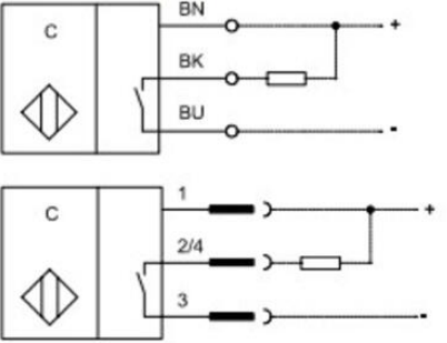
NPN - Proximity Switch
