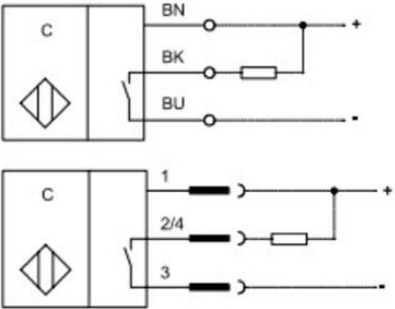
NPN - Proximity Switch
