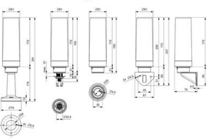
MT60 Dimension Drawing
