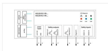
HOLDX_RL1_P8_1 standalone 8-pin pigtail without EDM function
