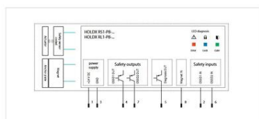
HOLDX_RL1_1 standalone 8-pin pigtail without EDM function
