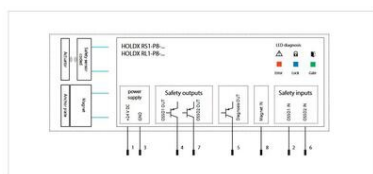
HOLDX_RL_1 standalone 8-pin pigtail without EDM function
