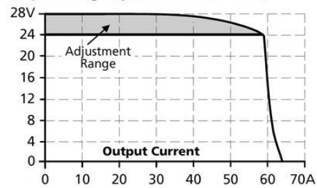
Output Voltage (dynamic behavior, < 12ms)
