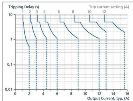
Fig. 6-1: CH1 and CH2 tripping diagrams in Slow mode
