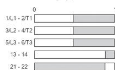
Auxiliary contacts
