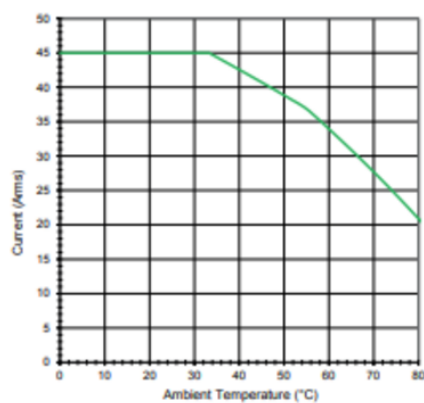
GNR+ - 45 A
