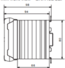
GNR+ 45 mm front view - GNR45DCZP
