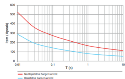
GNR+ - 45 A
