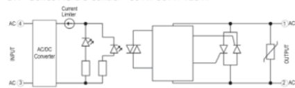
GN+ Series AC/DC control - 50 A / 90 A / 125 A
