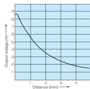
FRS8BC(reflective)
