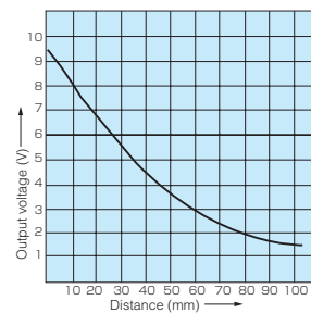
FTS5BC(through-beam)
