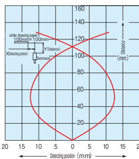
GN-R7C GN-R7CPN
