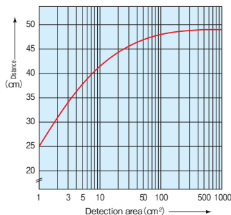
GN-R40CR GN-R40CRPN
