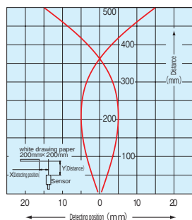
GN-R40CR GN-R40CRPN
