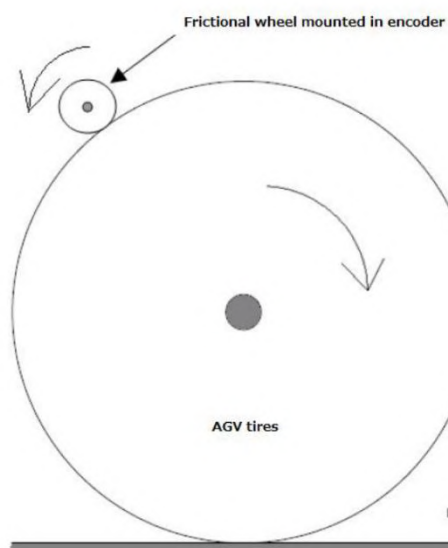
Figure 4-14 Calculation of pulse count per centimeter travel
