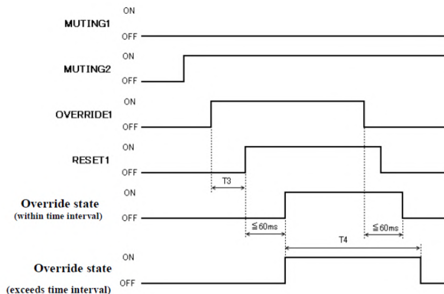
Figure 4-8 Override Sequence
