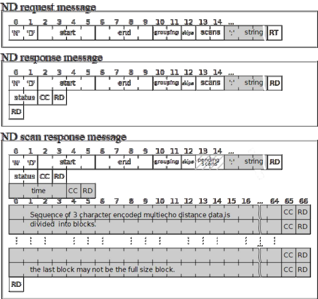
Figure 5.11.1: ND Message Format
