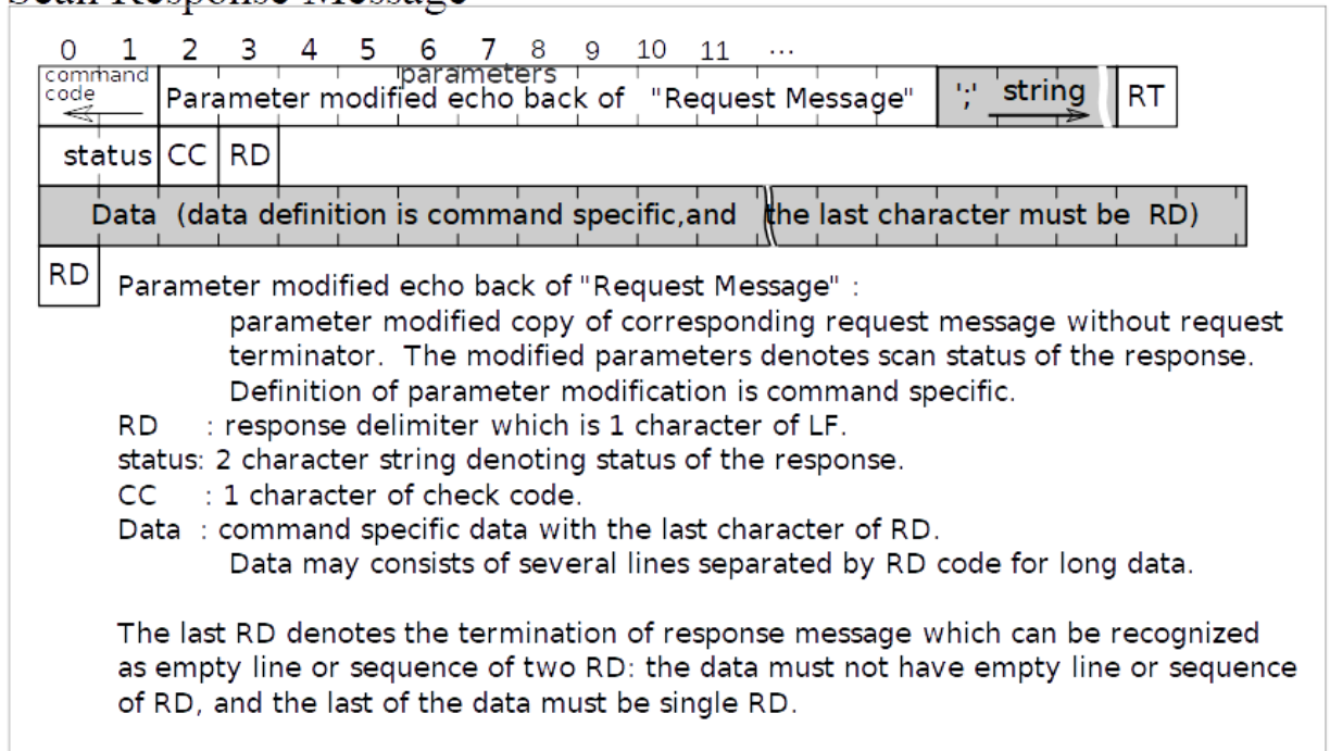
Figure 3.5.1 Scan Response Message Format
