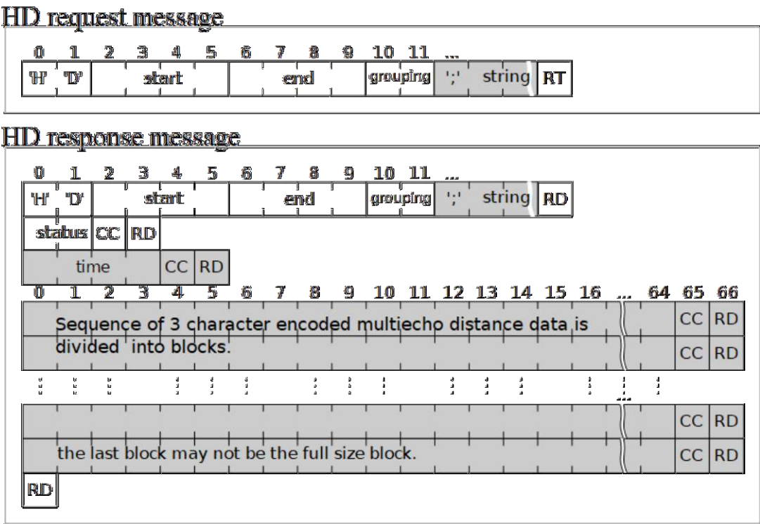
Figure 5.7.1: HD Message Format
