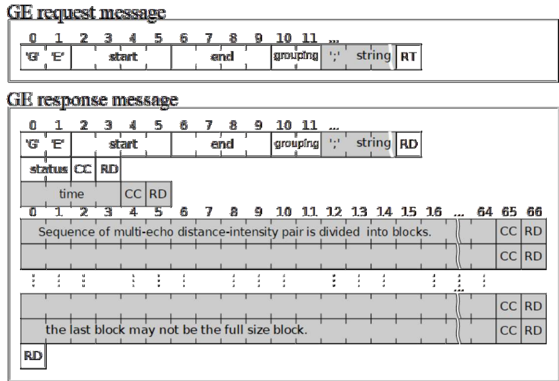
Figure 5.6.1: GE Message Format
