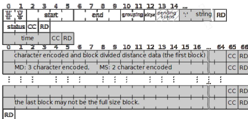
Figure 5.9.1: MD, MS Message Format
