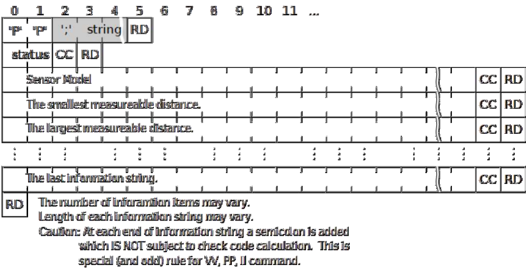
Figure 5.22.1: PP Message Format
