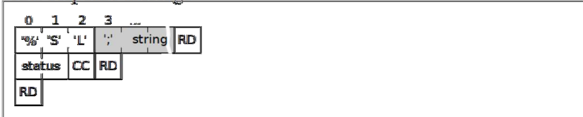
Figure 5.16.1: %SL Message Format
