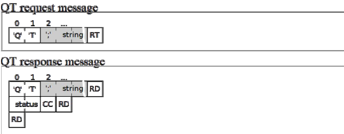
Figure 5.15.1: QT Message Format
