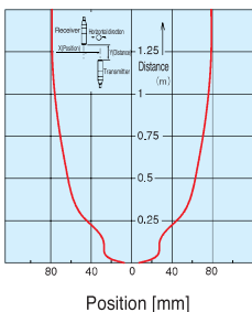
UX-T100D (PN)
